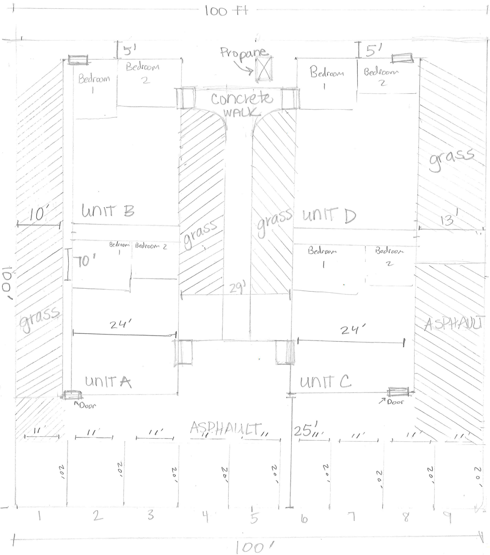
# 34 FOSTER SITE PLAN
